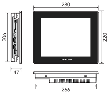
Panel cut
