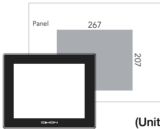
Panel cut
